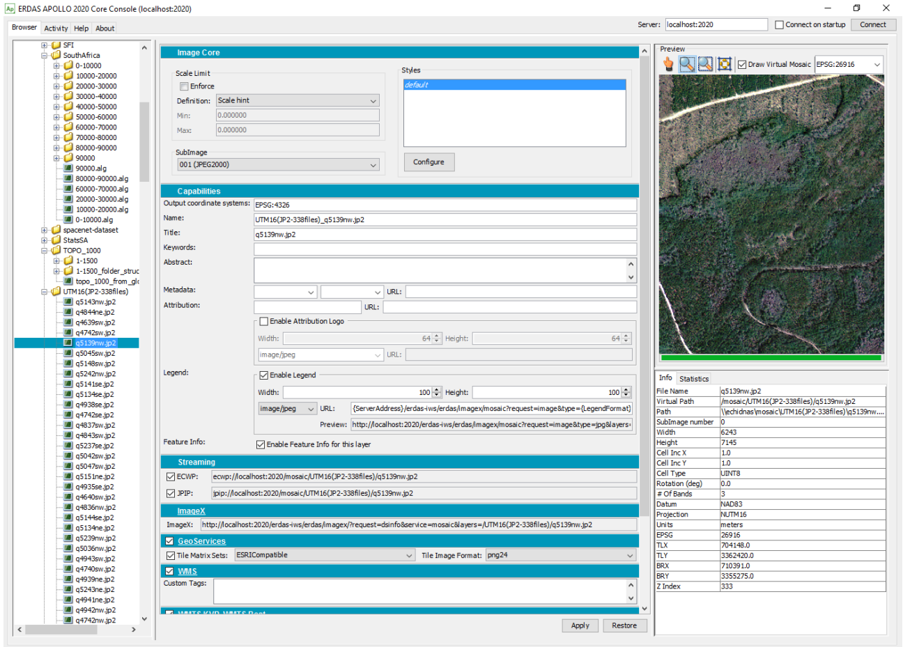
View data within the console to verify user experience
