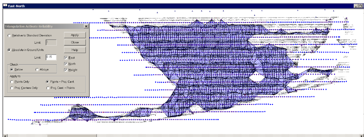
Effective footprints of the images showing coverage
